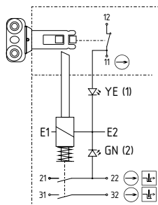
AZM190-02/01RKA AZM190-02/01RKA..-G LED付き
