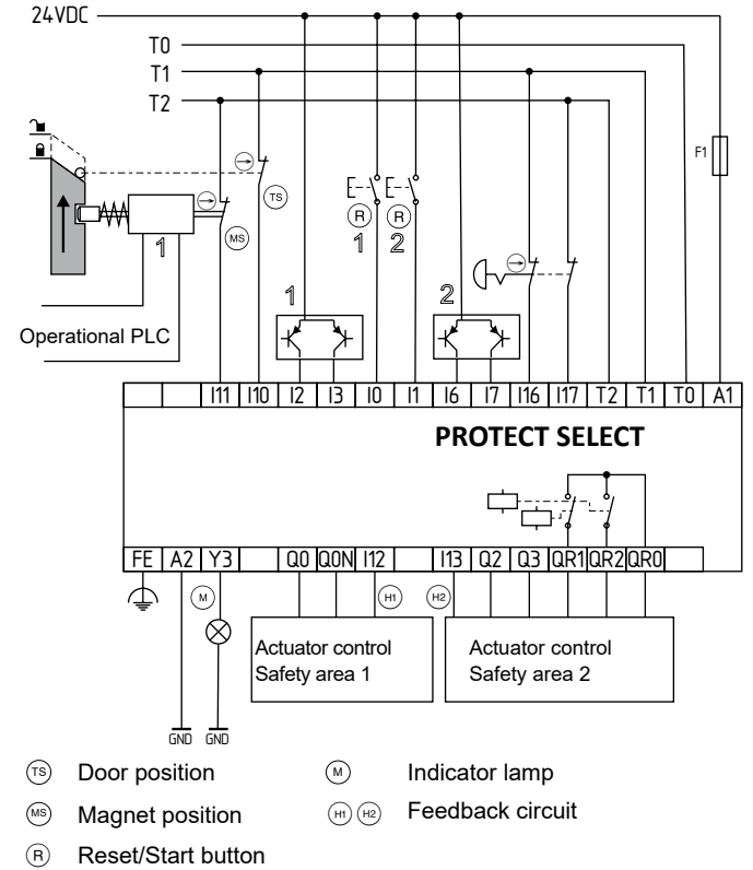
Wiring example:
