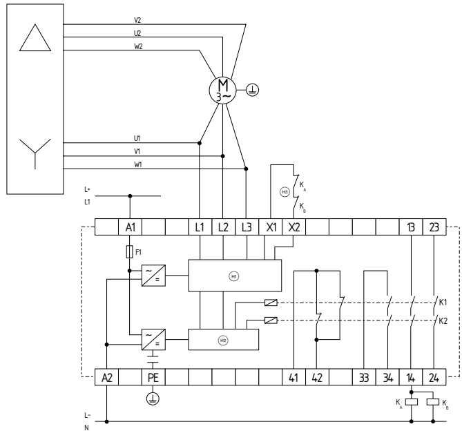
Fig. 3 (SP) = Signal processing (M) = Monitoring (FB) = Feedback circuit
